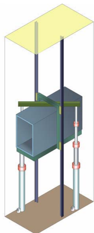
Side direct two cylinder
