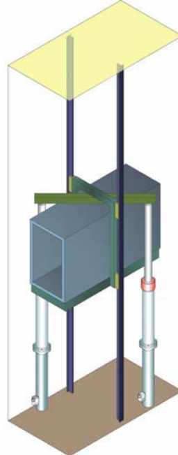
Side direct two cylinder
