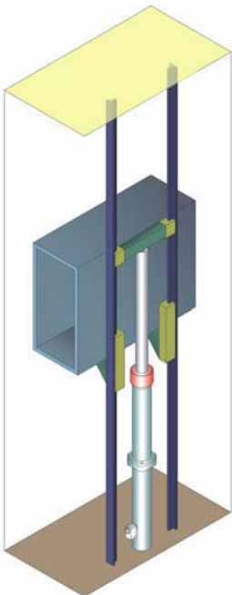
Side direct one cylinder
